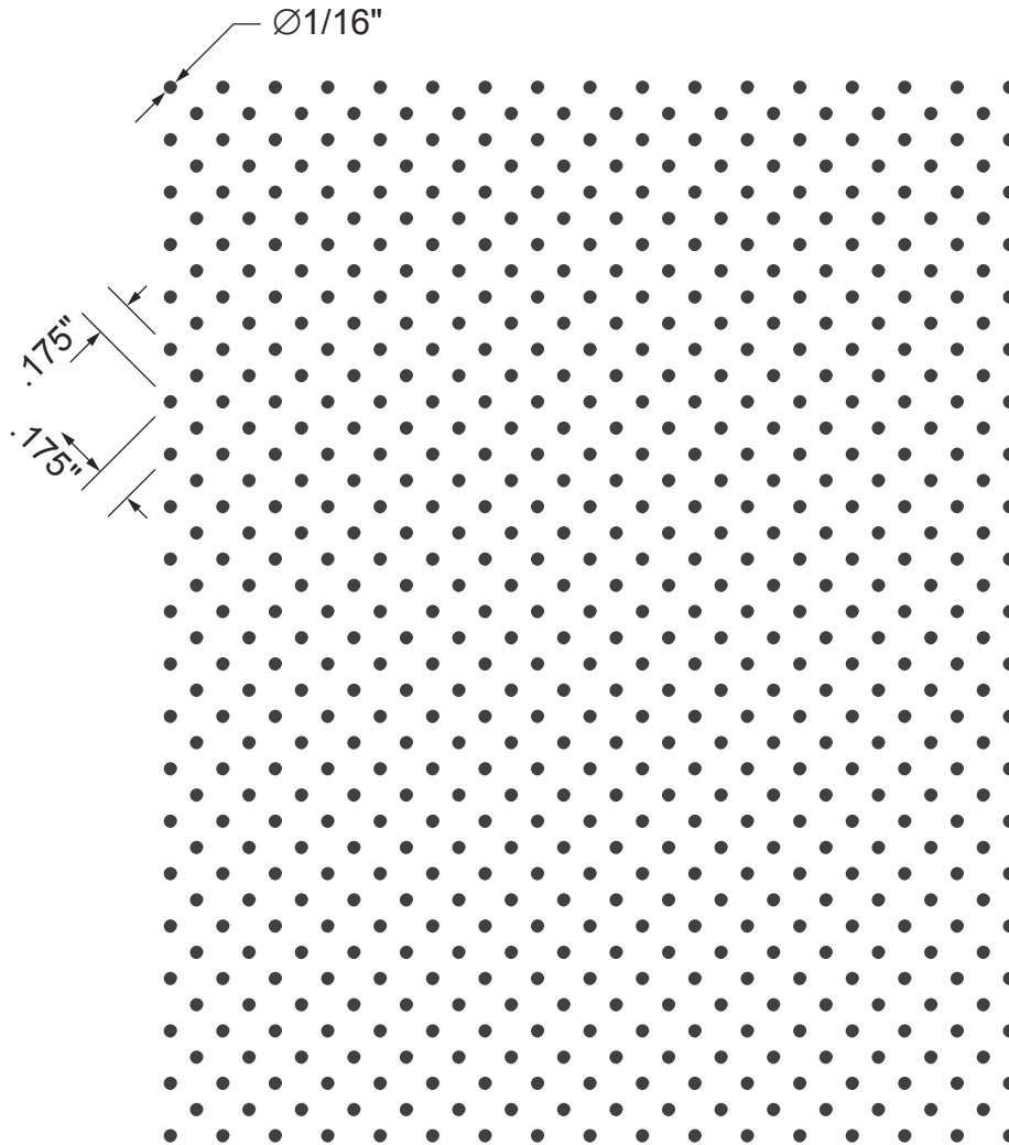
SD-7 1/16" Diameter @ .175" Diagonal Centers 10% Open
