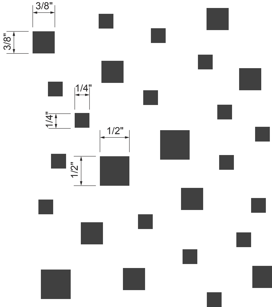
RN-36 1/4", 3/8" & 1/2" Square @ Random Centers 10% Open
