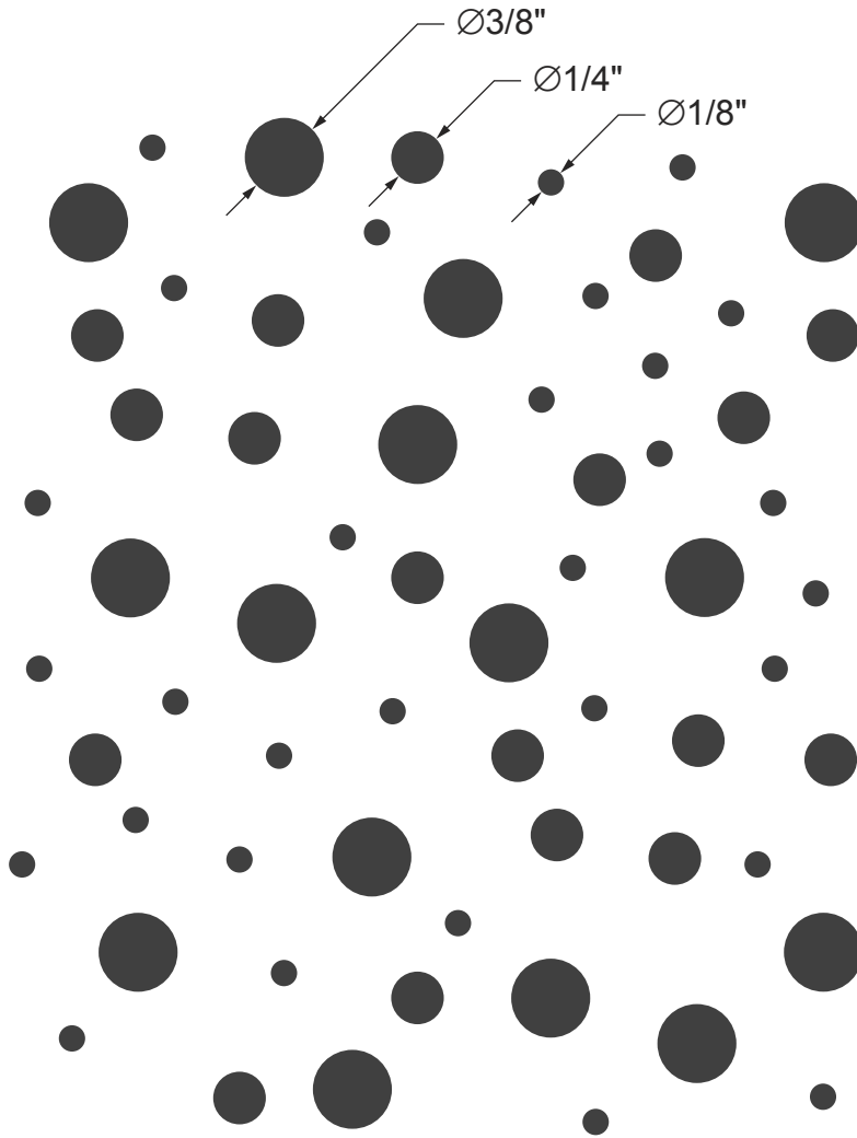
RN-10 1/8", 1/4" & 3/8" Diameter @ Random Centers 15% Open
