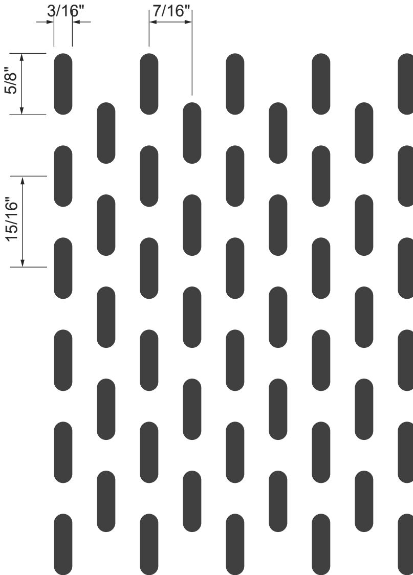
OB-19 3/16" x 5/8" Obround @ 7/16" x 15/16" Staggered Centers 27% Open
