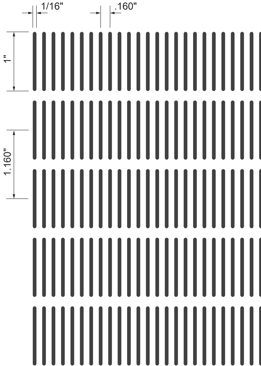
OB-15 1/16" x 1" Obround @ .160" x 1.160" Straight Centers 33% Open
