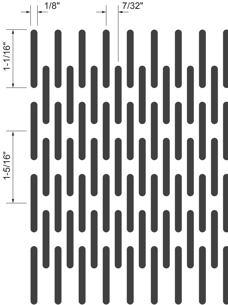
OB-12 1/8" x 1-1/16" Obround @ 7/32" x 1-5/16" Staggered Centers 45% Open
