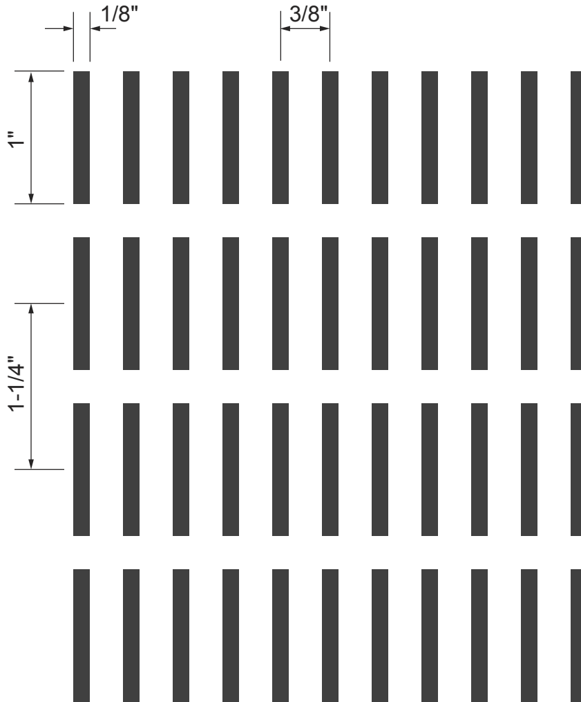
LT-40 1/8" x 1" Rectangular @ 3/8" x 1-1/4" Straight Centers 27% Open
