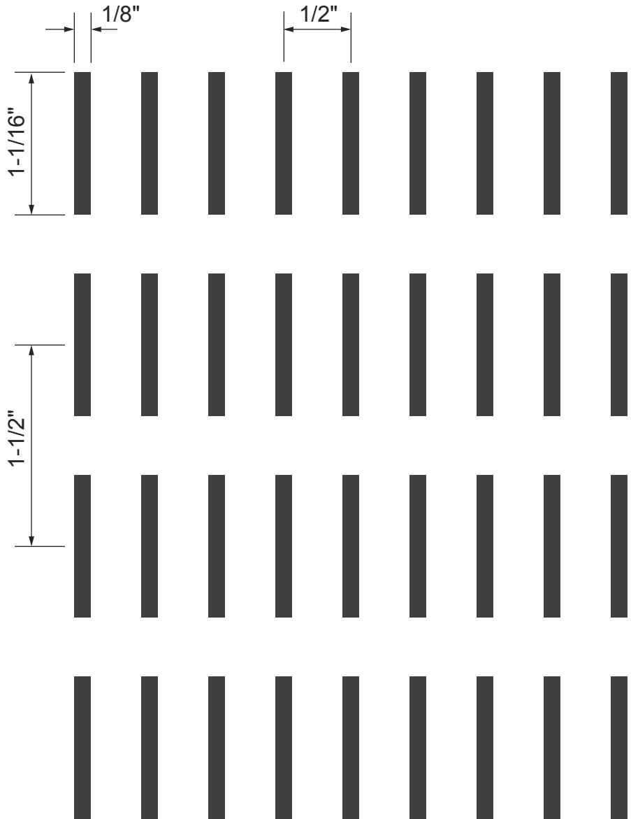
LT-39 1/8" x 1-1/16" Rectangular @ 1/2" x 1-1/2" Straight Centers 18% Open
