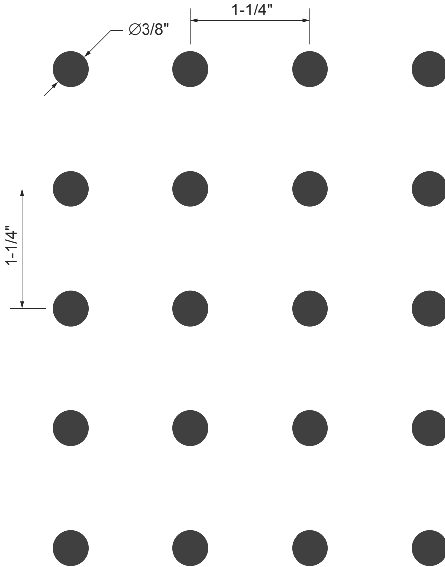
LT-29 3/8" Diameter @ 1-1/4" Straight Centers 7% Open
