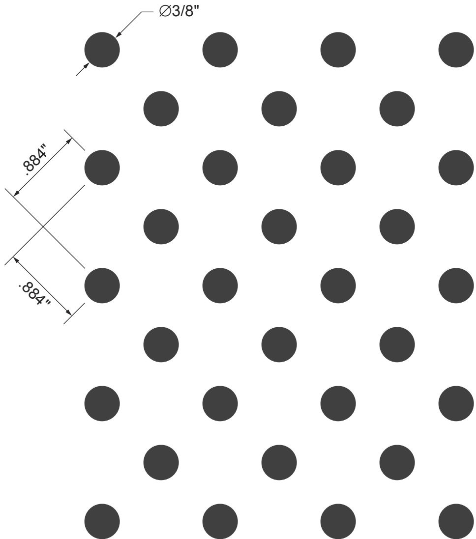
LT-27 3/8" Diameter @ .884" Diagonal Centers 15% Open
